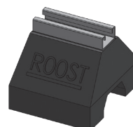
FIG. 7500 Series Rooftop Support Block 5" STRUT CHANNEL: Pre-Galv, 13/16" X 1-5/8"
